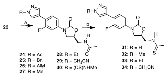
Scheme 3. Reagents: (a) RBr or RCOCl, base, THF or acetone, reflux, 21–94%, or NaH, DMF, 0 °C then CH 3 NCS, 43%; (b) Lawesson's reagent, THF, reflux, 32–94%.
