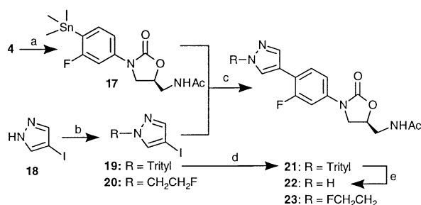
Scheme 2. Reagents: (a) (Me 3 Sn) 2 , PdCl 2 (PPh 3 ) 2 , dioxane, reflux, 99%; (b) Trityl-Cl, Et 3 N, DMF, >90% or NaH, DMF; BrCH 2 CH 2 F, 80%; (c) 19 or 20 , Pd 2 (dba) 3 , TFP, LiCl, NMP, 90 °C (0–40%); (d) Diboron pinacol ester, KOAc, Pd(PPh 3 ) 4 , DMF, 100 °C then 4 , Pd(PPh 3 ) 4 , Na 2 CO 3 , 100 °C; (e) TFA, CH 2 Cl 2 , 53–76% for steps d and e to give 22 .
