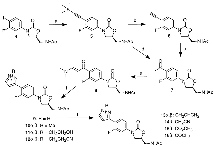
Scheme 1. Reagents: (a) TMSCH 2 CH 2 , Pd(PPh 3 ) 2 Cl 2 , CuI, Et 3 N, DMF, 45 °C, 99%; (b) K 2 CO 3 , CH 3 OH, 60% (c) HgO, Nafion, H 2 O, CH 2 Cl 2 , reflux, 20% or formic acid, 85 °C, 57%; (d) formic acid, 95 °C, 69%; (e) Me 2 NCH(OMe) 2 , EtOH, reflux, 76%; (f) H 2 NNHR, EtOH reflux to yield 62–97% of 9 , 10 ( \alpha/\beta = 6:1), 11 ( \alpha/\beta = 7:1), 12 ( \alpha/\beta = 10:1); (g) NaH, DMF, 0 °C then RBr or RCOCl to yield 26–94% of 13 ( \alpha/\beta = 1:8), 14 \beta , 15 \beta and 16 \beta .
